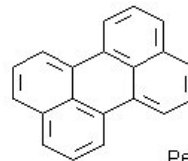
Perylene
